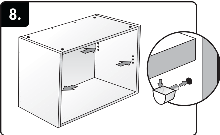
Insert shelf studs into the side panels.
